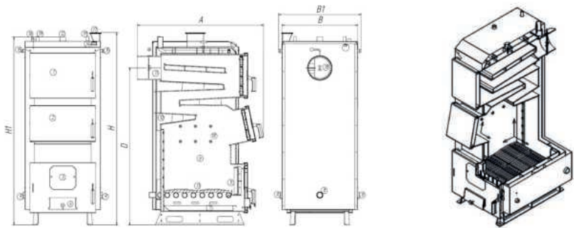
Рис.2 Vulcan VPSFW 60, VPSFW 70
